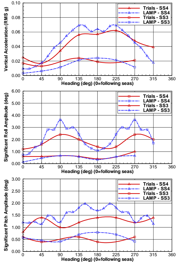
Figure 8 LAMP vs. Trials Data: 15 knots, SS3 & SS4
