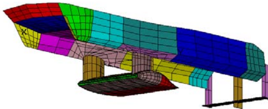
Figure 3 Sea Flyer Geometry Model
