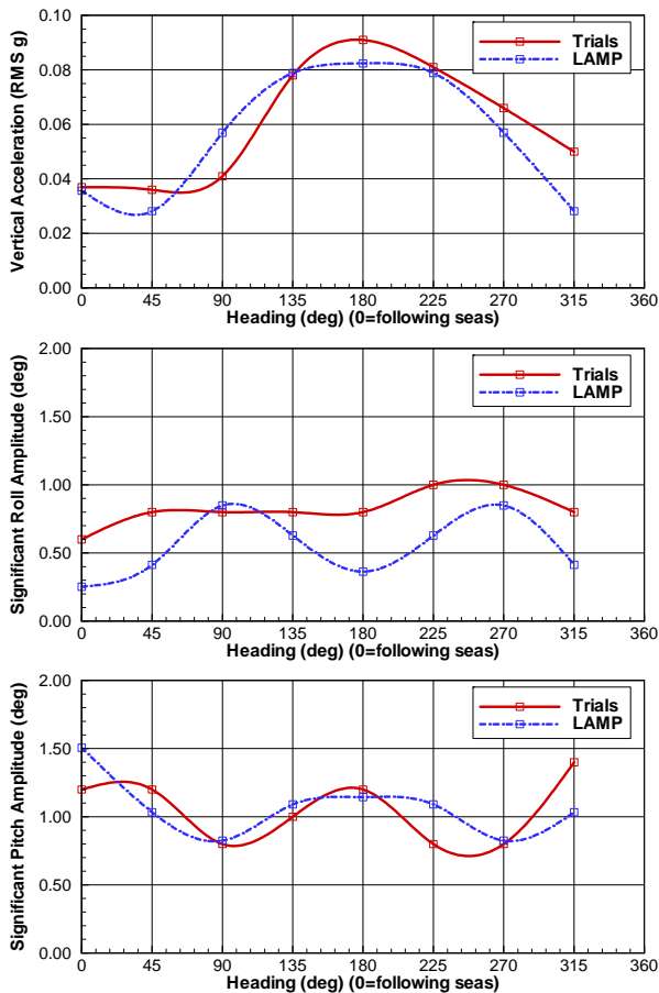
Figure 7 LAMP vs. Trials Data: 27 knots, SS4
