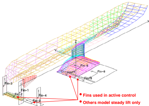
Figure 6 Appendage Model for LAMP Simulations
