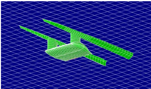
Figure 4 Hull and Local Portion of the Free Surface Panel Grid
